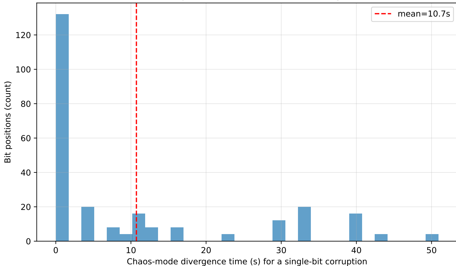
Pendulum 1-bit perturbation \rightarrow O(1) state divergence time
