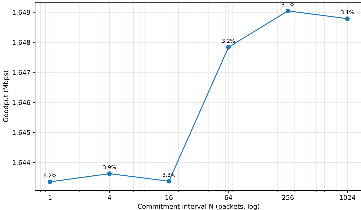
CEP goodput vs HMAC commitment interval N (labels = overhead%)
