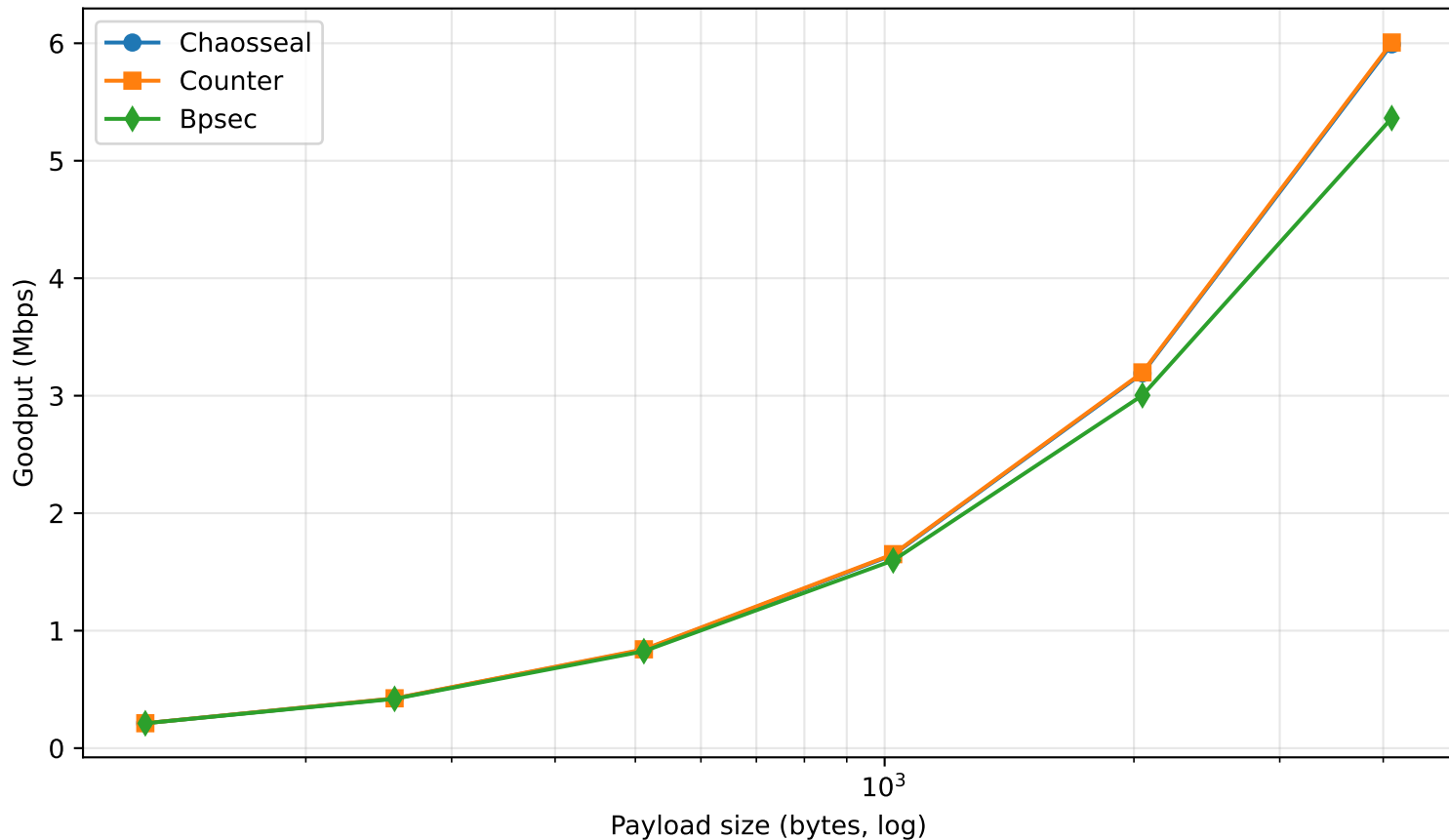
CEP vs counter vs BPsec — goodput vs packet size
