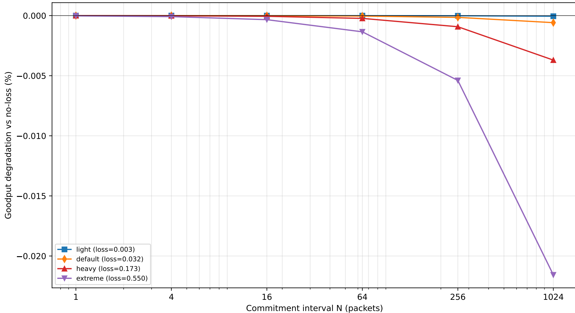
Relative Goodput Degradation Due to Burst Loss (Lower N = more frequent HMAC = faster desync detection)
