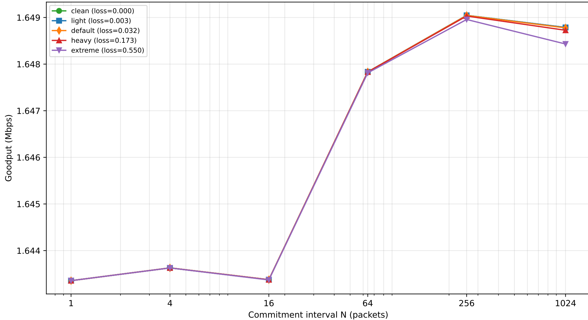
CEP Goodput vs HMAC Commitment Interval Under Different LEO Loss Profiles
