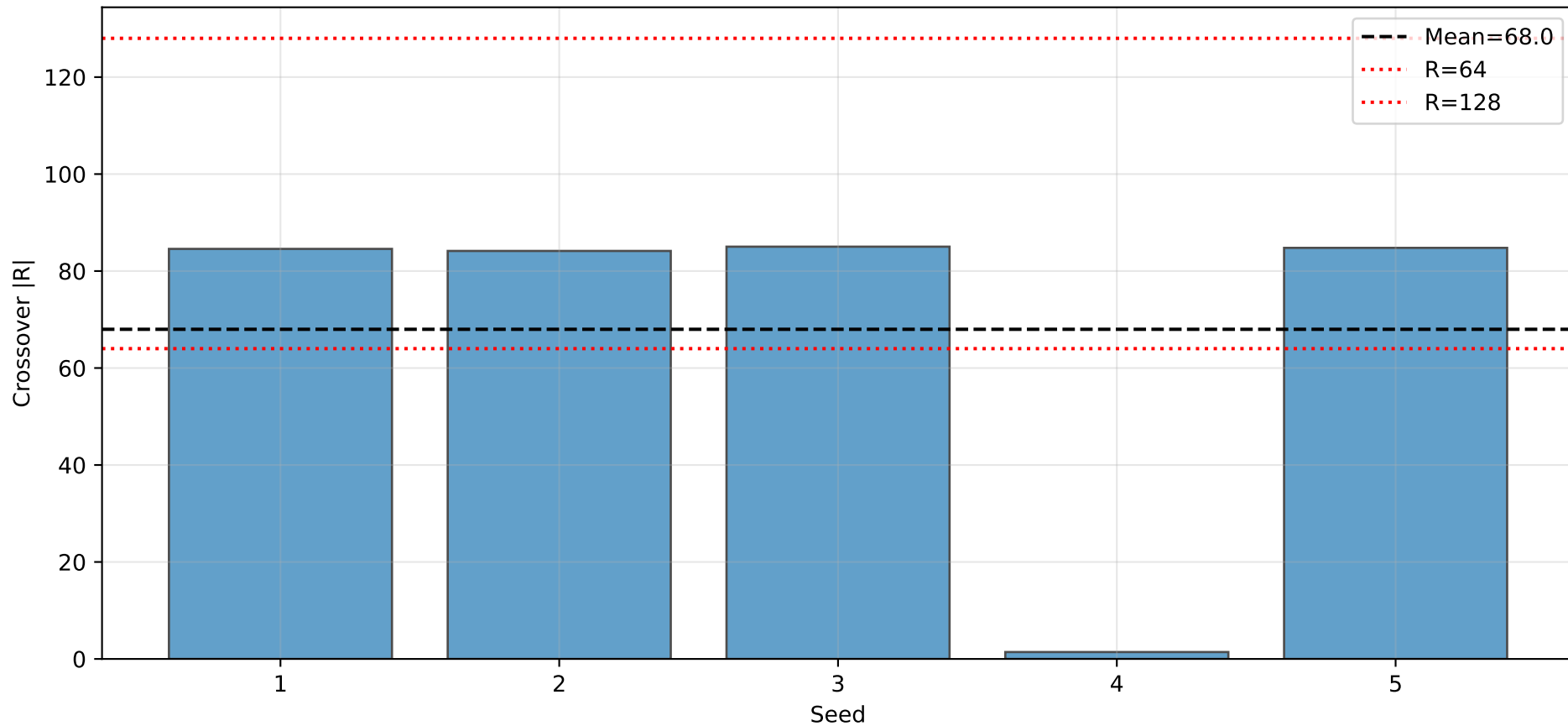
Per-Seed Crossover Point (R where CEP goodput = BPSec)
