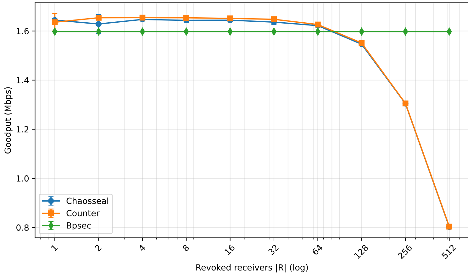
CEP (pendulum) vs counter baseline vs BPsec — goodput vs |R|
