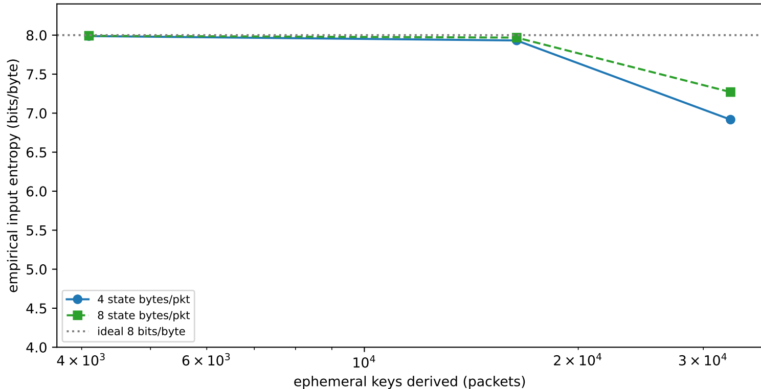
Per-packet key-derivation input entropy from chaotic trajectory
