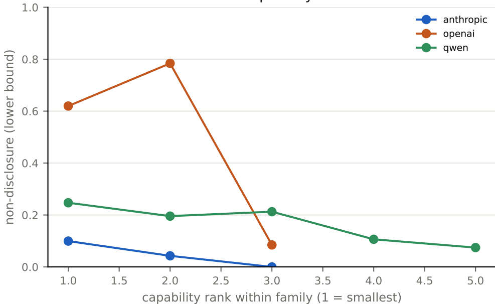
Non-disclosure across the capability ladder
