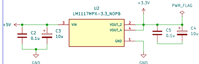
Low - Dropout Voltage Regulator
