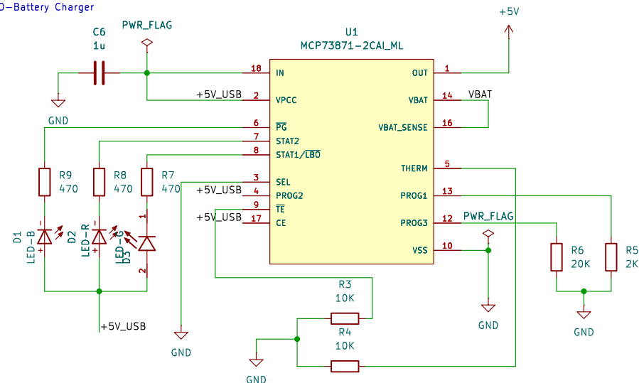
LIPO-Battery Charger
