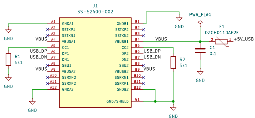
USB-C connector
