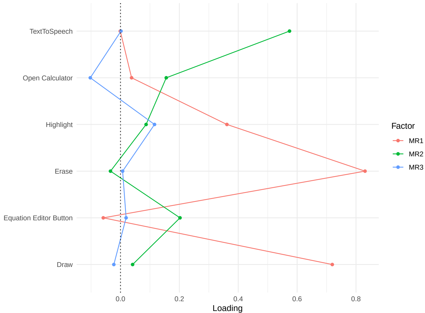
Item 7 Factor Loadings
