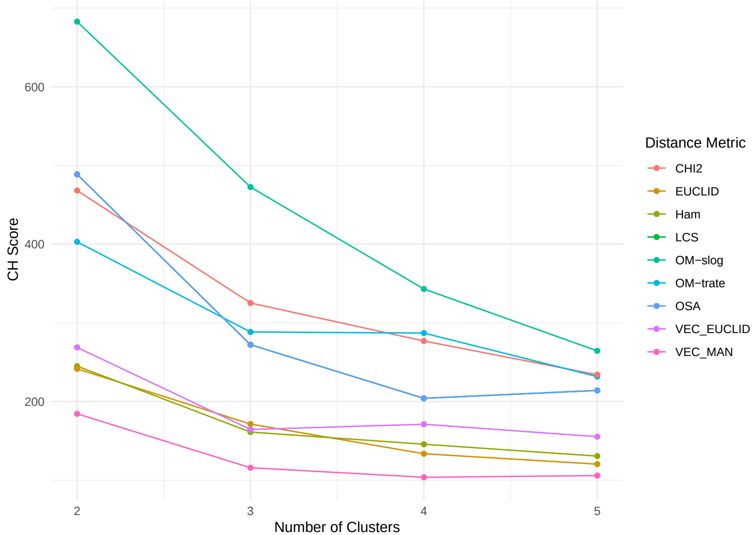
Calinski–Harabasz Index by Distance Metric
