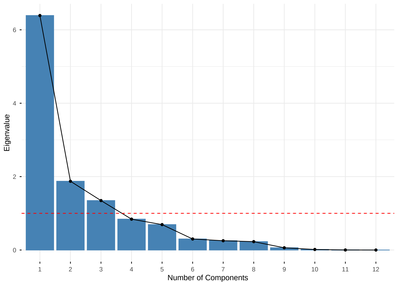
Scree Plot of Eigenvalues for Sequence Metrics Principal Components
