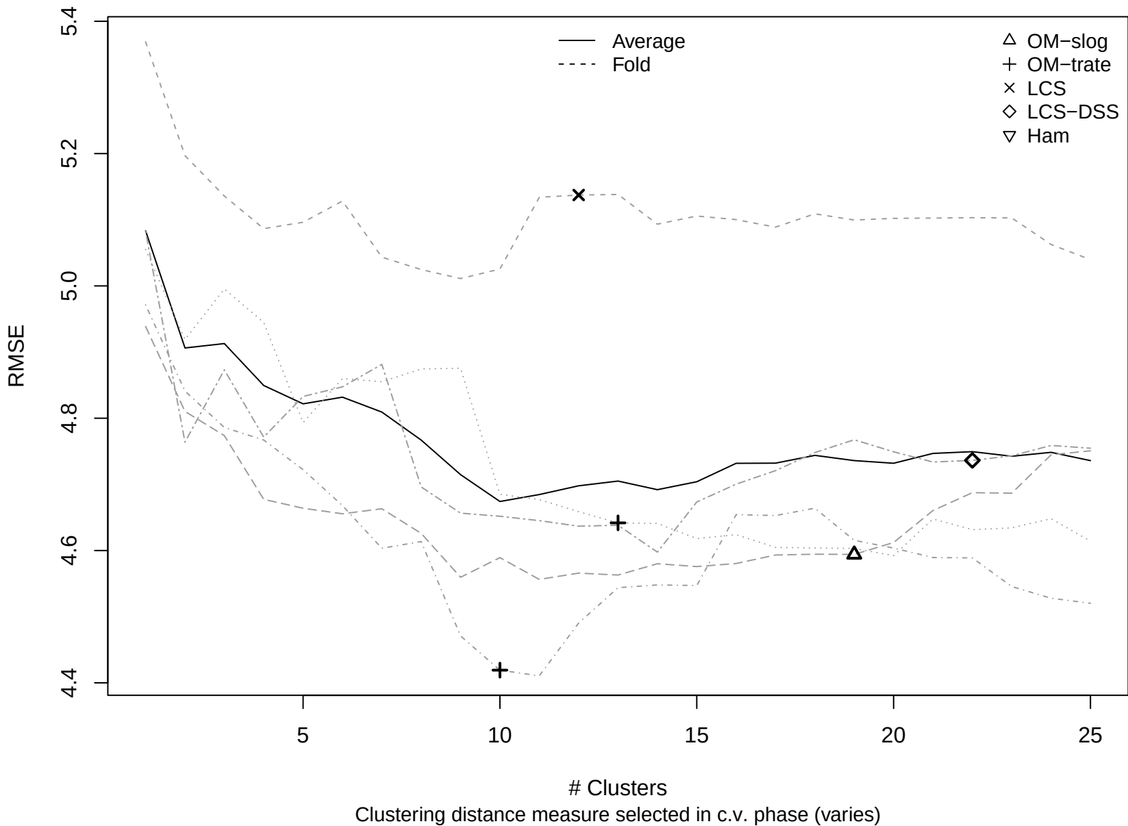
Cross-validated selection of number of components evaluated on withheld samples
