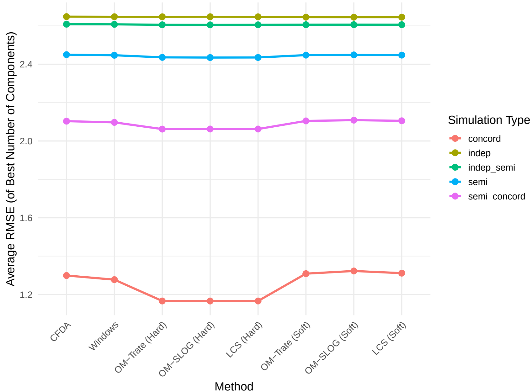
Mean RMSE per Method – Easy Difficulty
