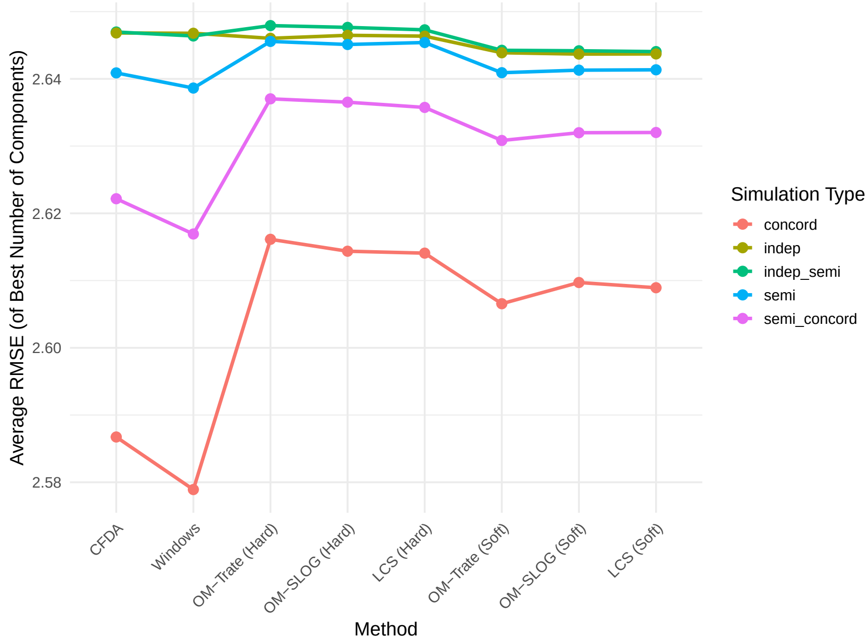
Mean RMSE per Method – Very Hard Difficulty
