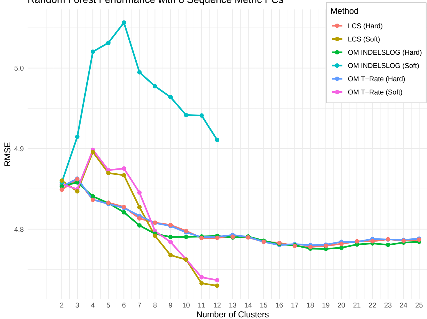
Random Forest Performance with 8 Sequence Metric PCs
