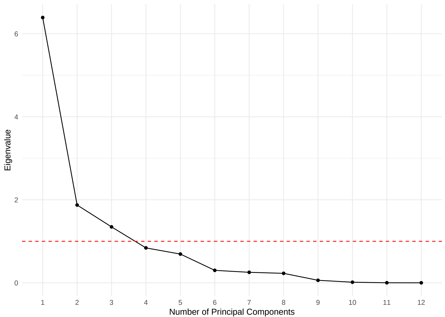
Scree Plot for Sequence Metrics
