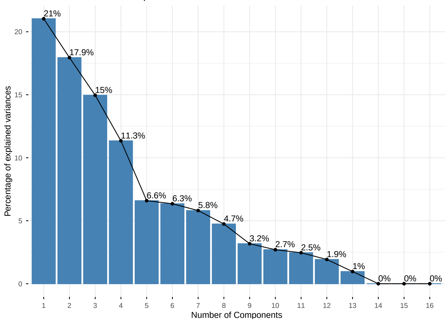
Scree Plot of Variance Explained for Windows Counts
