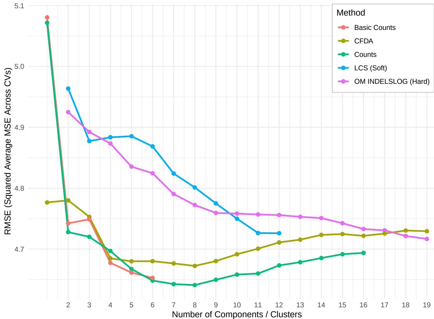
Random Forest Performance
