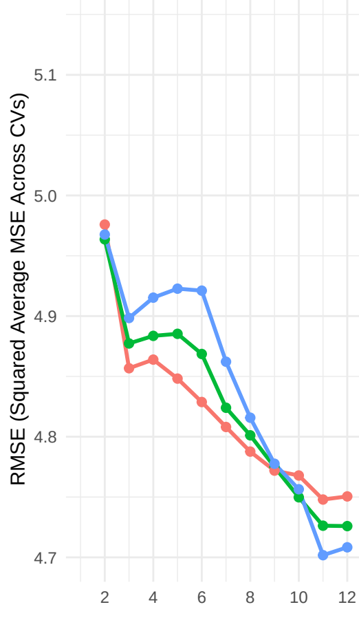
LCS (Soft)
