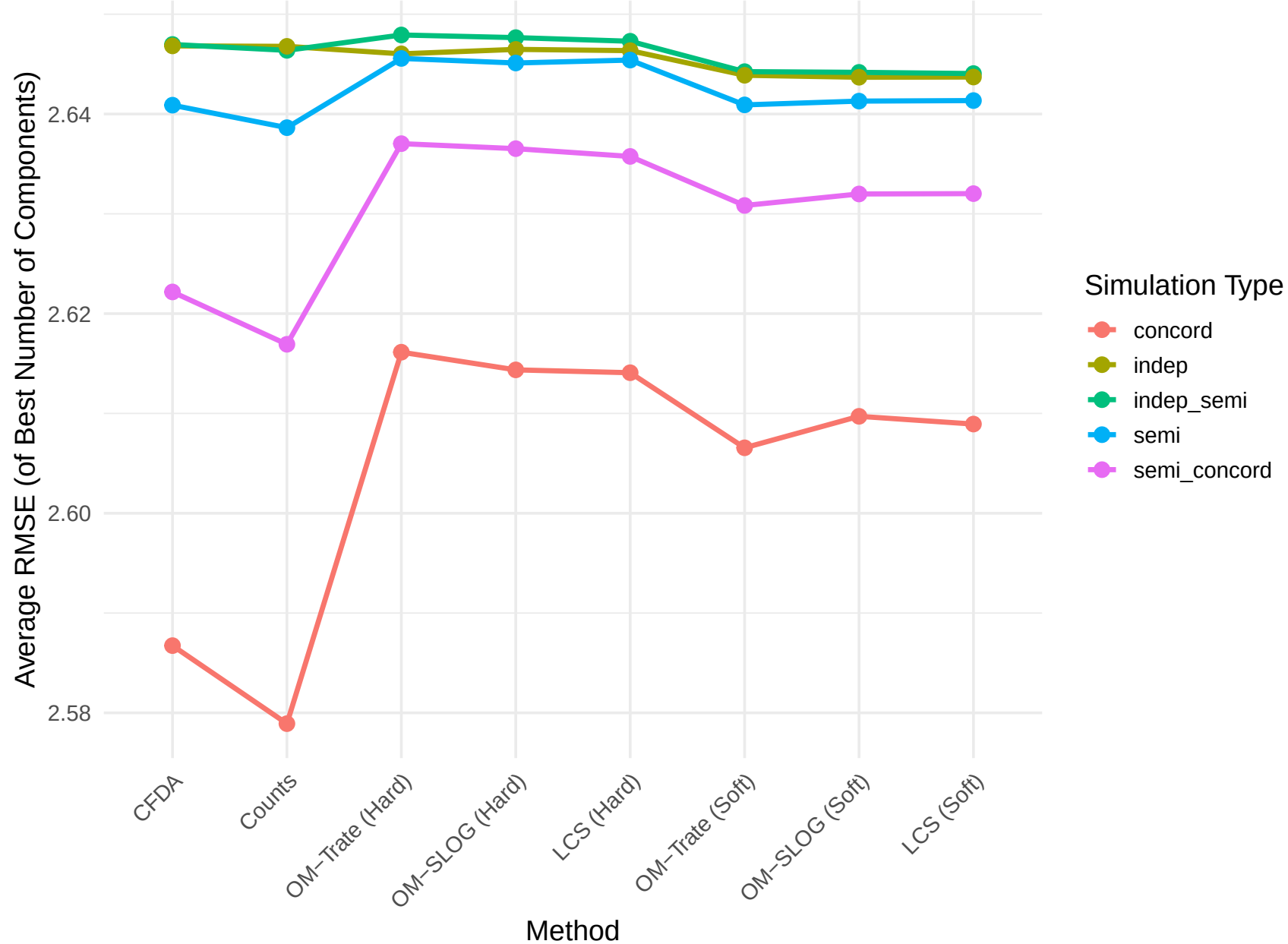
Mean RMSE per Method – Hard Difficulty
