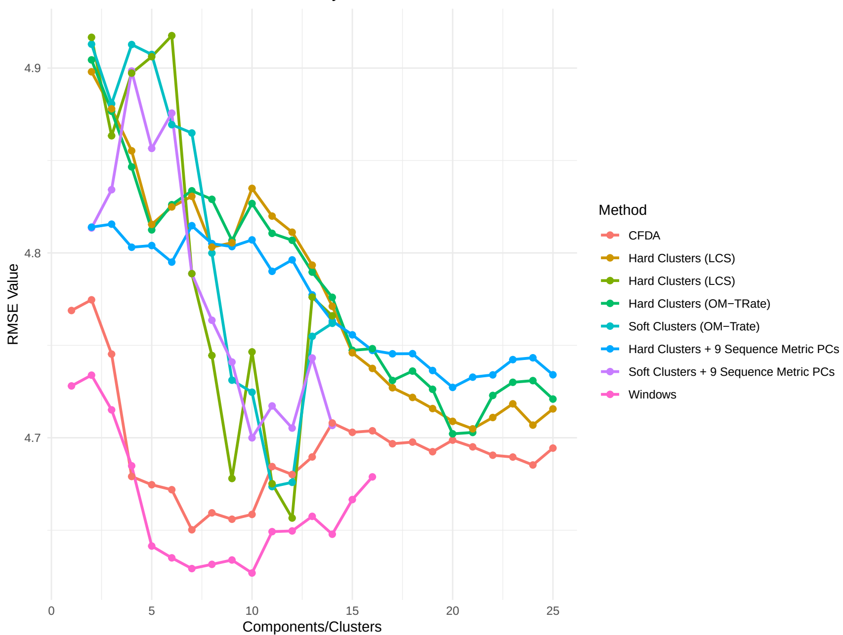
Random Forest Tuned Performance by Method
