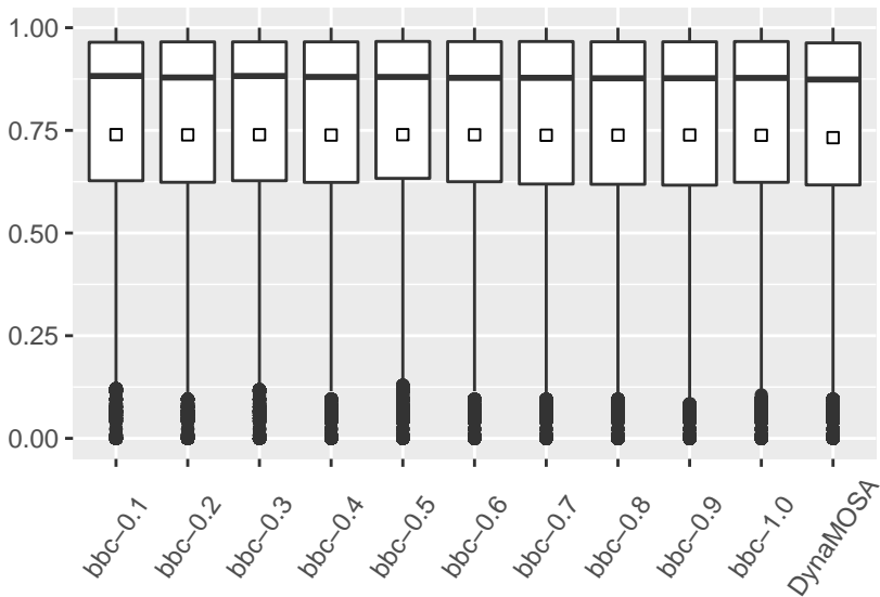
Weak mutation score
