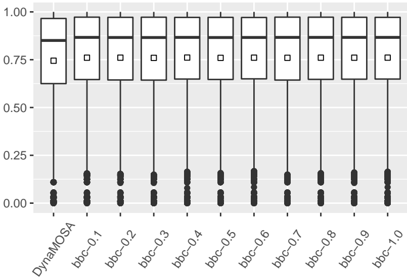
Branch coverage
