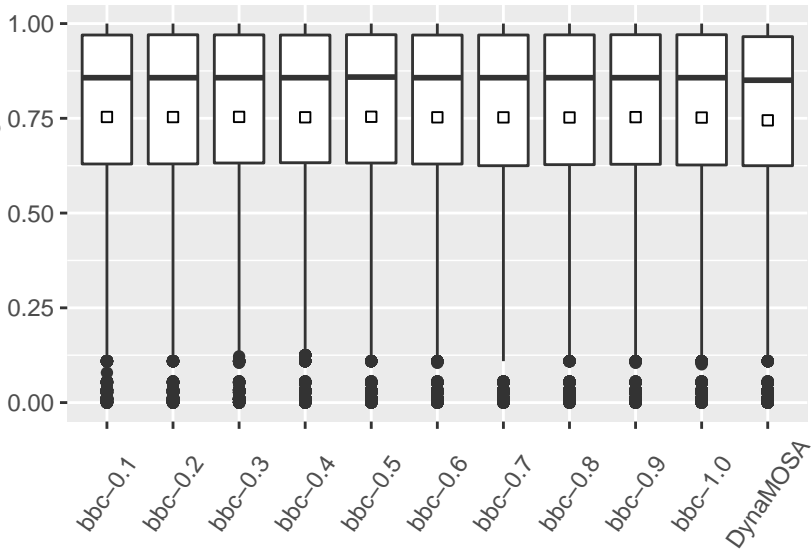
Branch coverage
