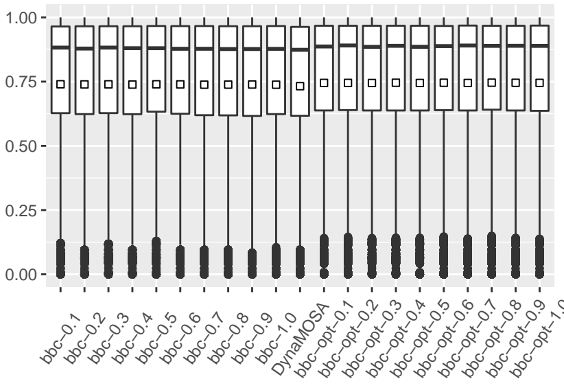
Weak mutation score
