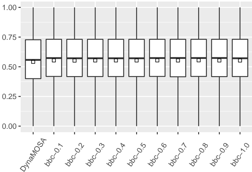
Output coverage
