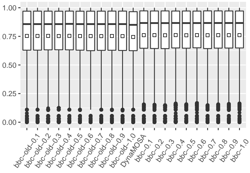
Branch coverage
