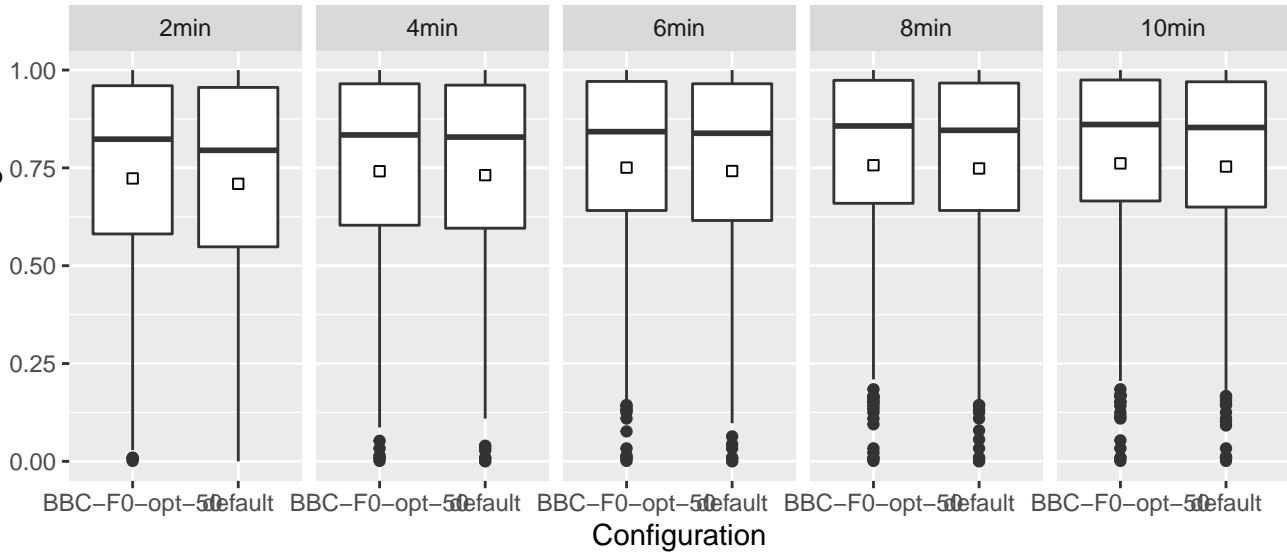
Branch Coverage
