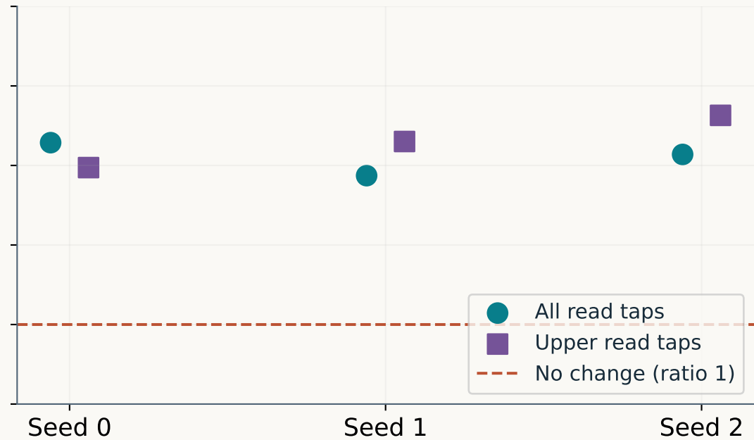
CounterFact
