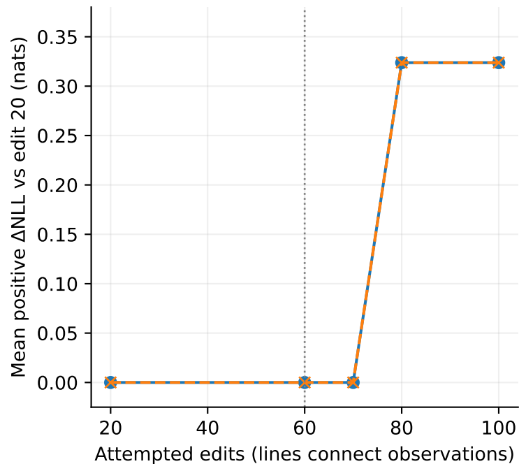
counterfact · exact old answers 20/20
