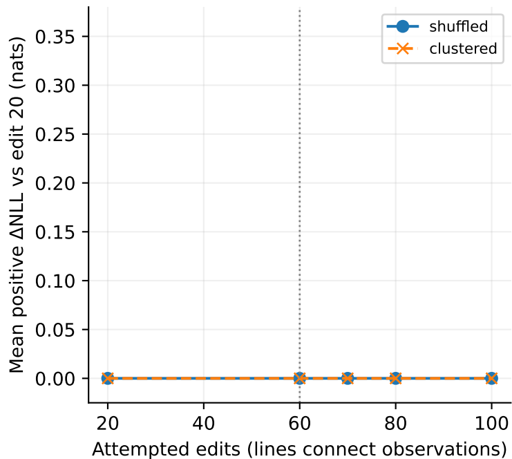
zsre · exact old answers 20/20
