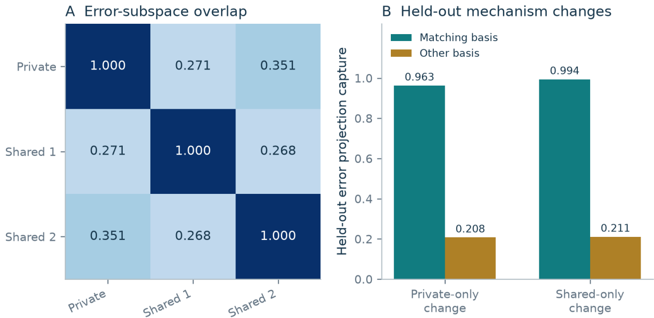
Figure 5. P4 uses 8,192 vectors per cause kind, six block outputs, width 128 and rank-16 bases. A: mean subspace overlap (diagonal is 1 by definition); independent random rank-16 subspaces would have expected overlap 16/128 = 0.125 , a reference value rather than a significance test. B: held-out projection capture for matching and nonmatching mechanism changes, averaged over layers [8].
