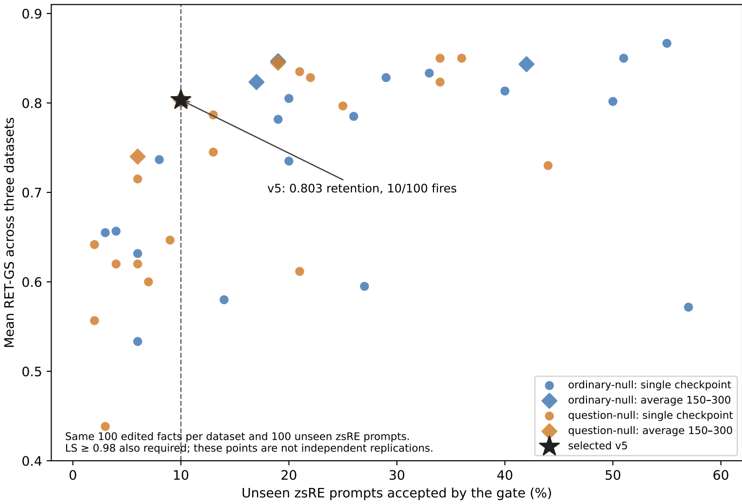
Development retention-rejection trade-off: 42 candidates
