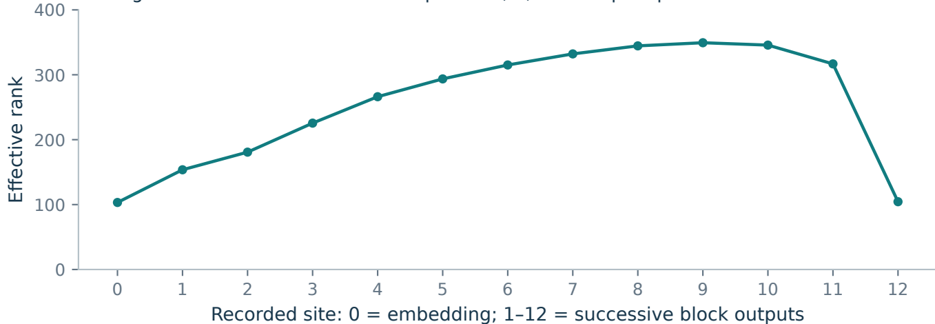
P2: regenerated ePC hidden-feature spectrum, 4,096 sampled positions
