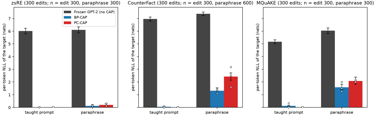
Figure 1: Ordinary adaptation: per-token loss
