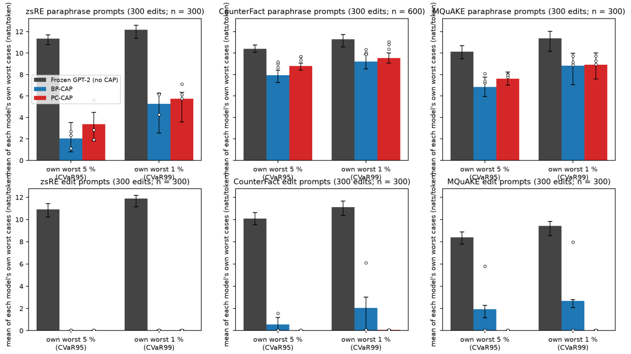
Figure 3: Own worst cases
