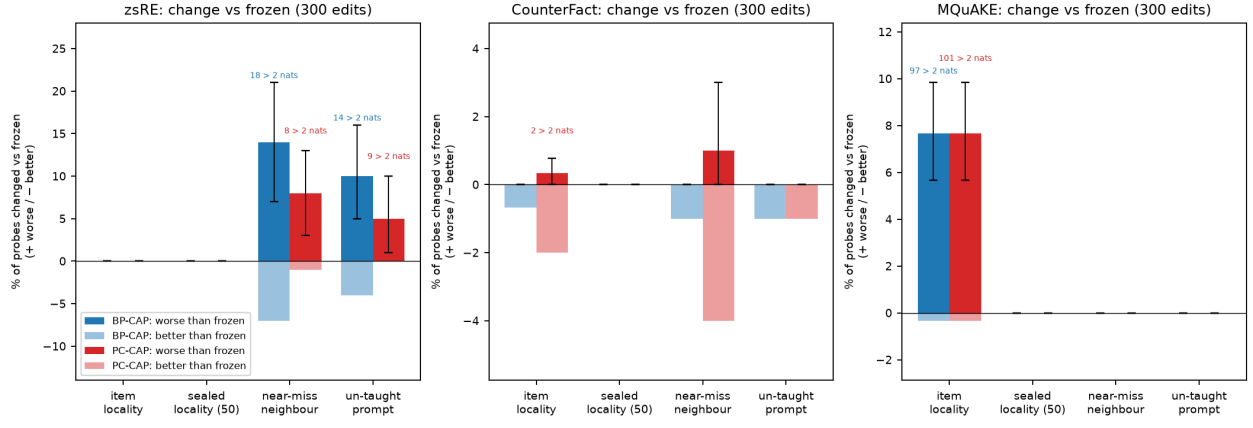
Figure 10: Collateral change vs frozen
