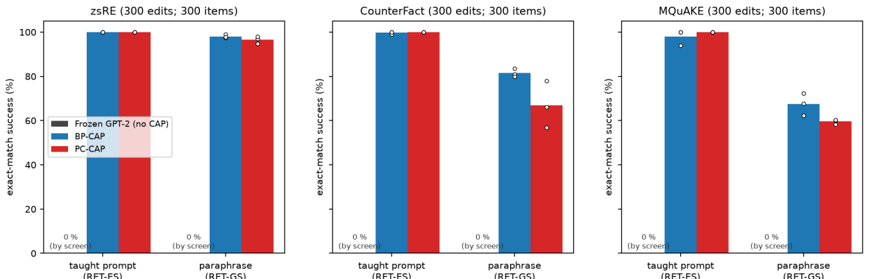
Figure 2: Ordinary adaptation: exact-match success
