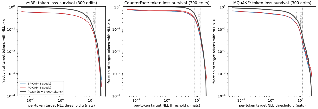
Figure 9: Token-loss survival
