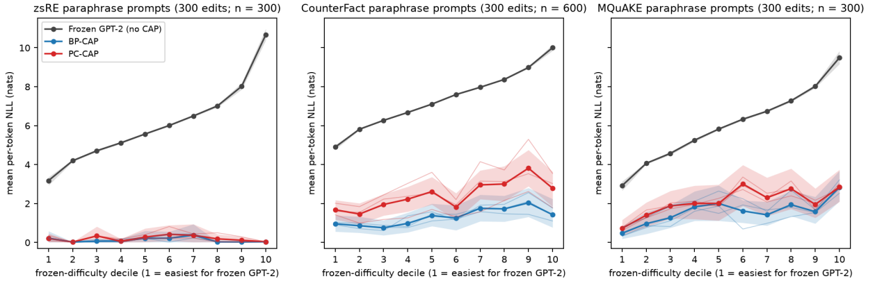
Figure 5: Deciles, paraphrase
