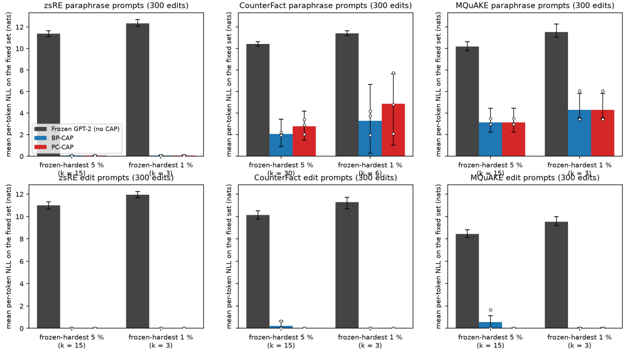
Figure 4: Frozen-hardest sets
