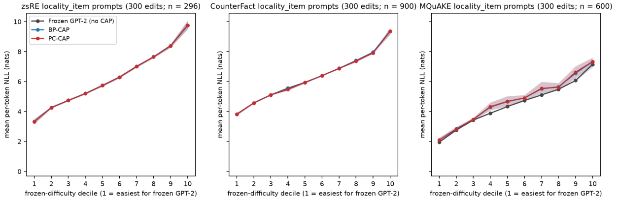
Figure 8: Deciles, item locality
