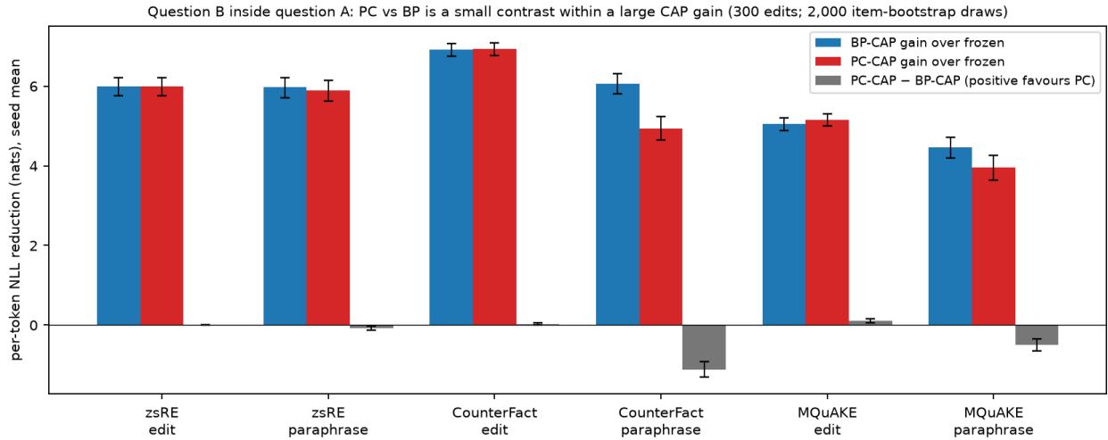
Figure 12: PC vs BP inside the CAP gain
