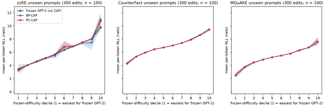
Figure 7: Deciles, un-taught prompt
