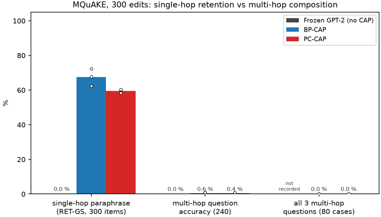
Figure 11: MQuAKE multi-hop
