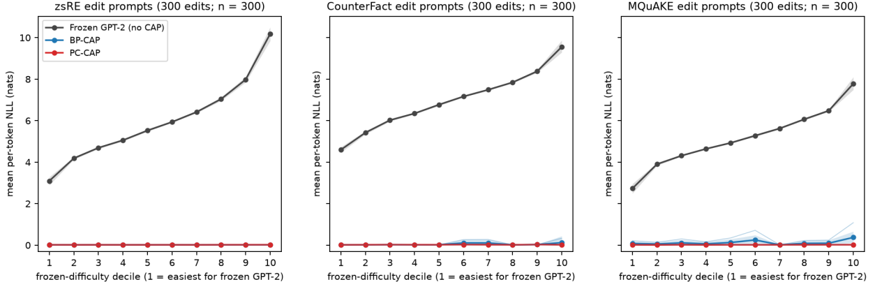
Figure 6: Deciles, taught prompt
