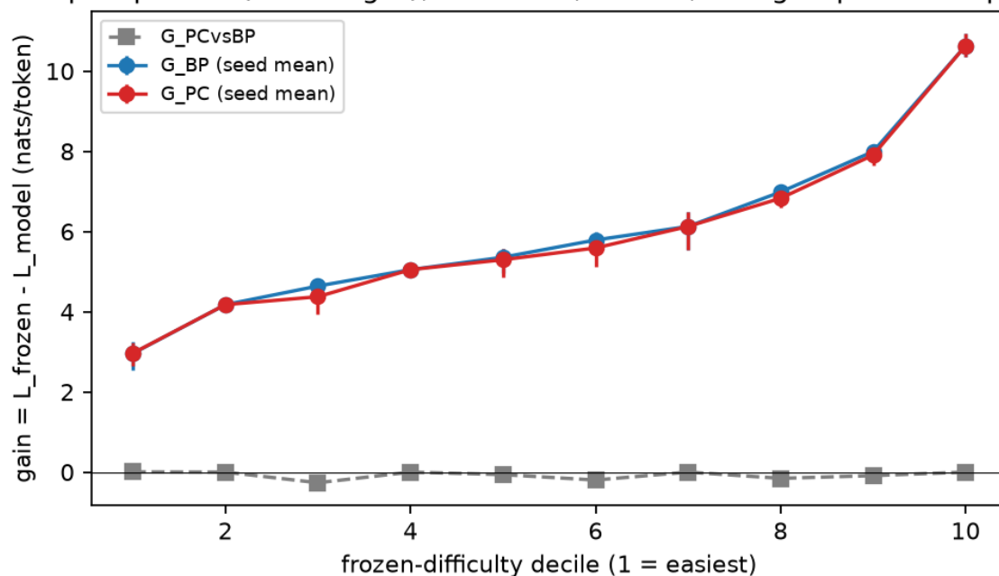
Figure 6: Deciles, zsRE paraphrase
