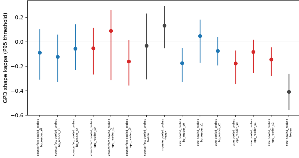
Figure 4: GPD shapes of per-probe target loss
