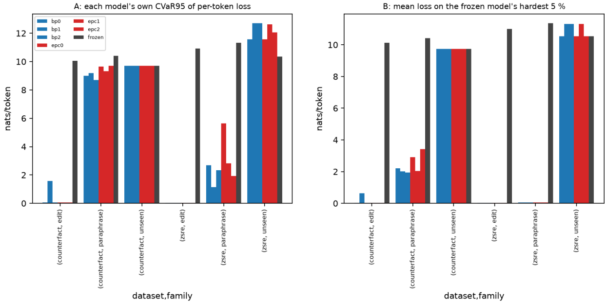
Figure 8: CVaR A and B
