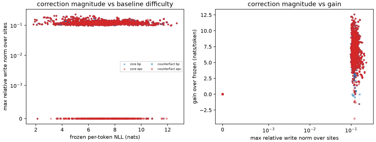
Figure 9: Write norms vs difficulty and gain
