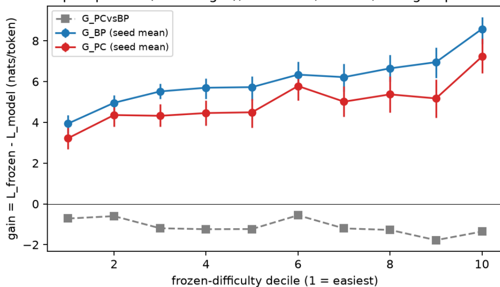
Figure 7: Deciles, CounterFact paraphrase
