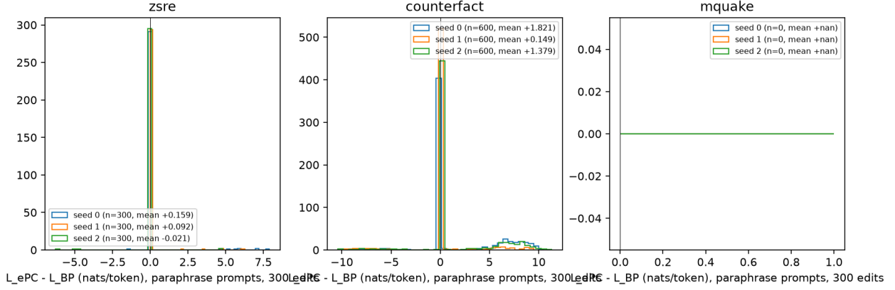
Figure 5: Paired ePC – BP differences on paraphrases
