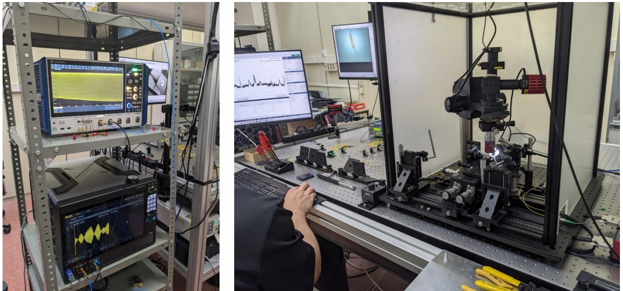
Image 1. Optomechanics laboratory at ICMM-CSIC ( Lab 047 at ICMM). Left: time and frequency-domain characterization rack (oscilloscope, spectrum analyzer, arbitrary waveform generator). Right: fiber-taper coupling station for interrogating photonic crystal cavities.
