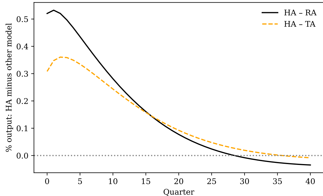
IRF of output inequalities across models
