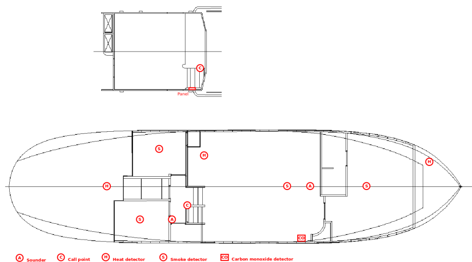
Figure 6. Fire alarm system
