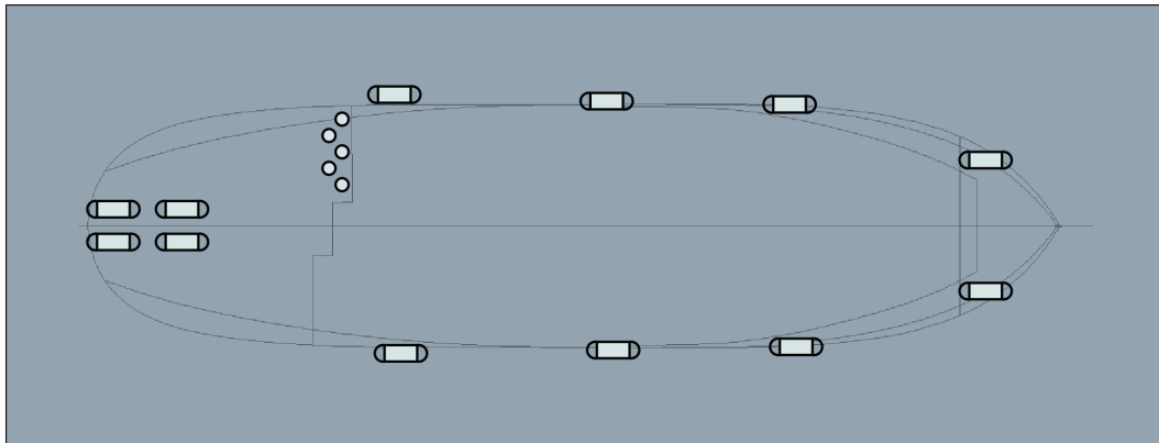
Figure 3. Location of anodes
