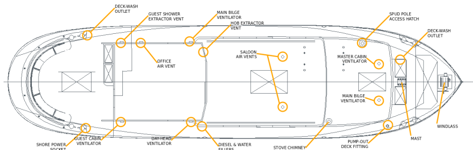
Figure 12. Deck equipment
