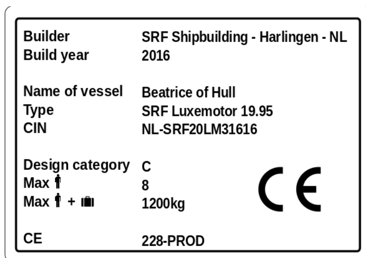
Figure 2. Builders plate
