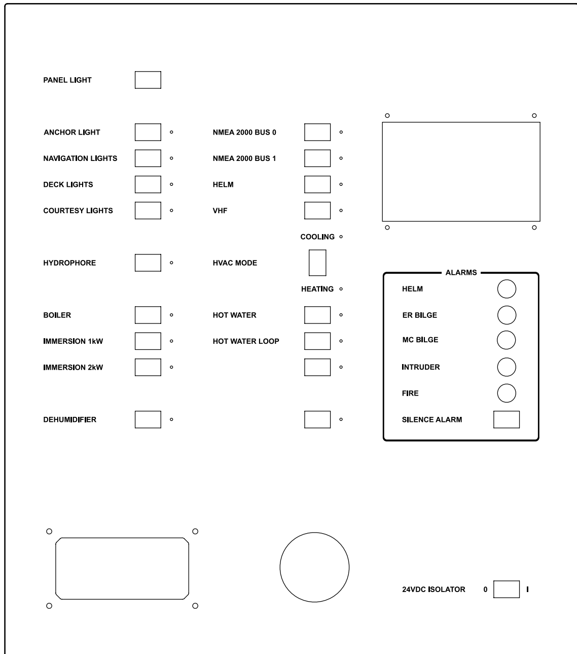
Figure 13. Domestic panel layout
