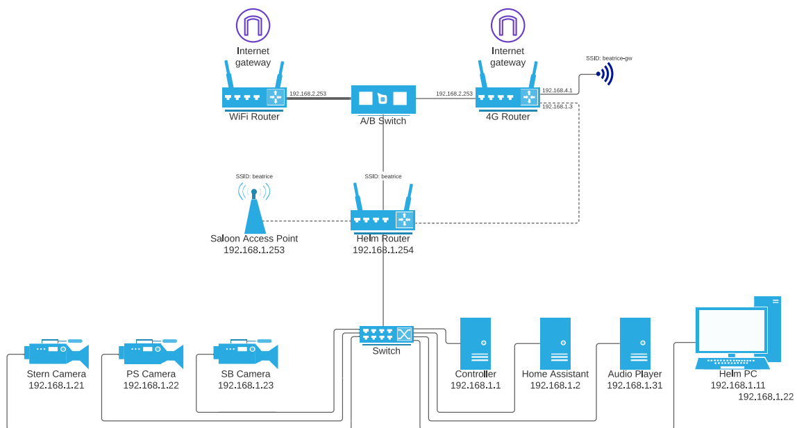
Figure 16. Schematic of Beatrice's Ethernet LAN
