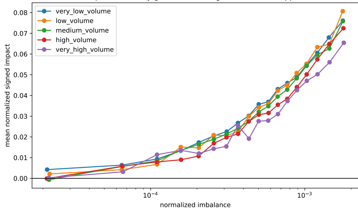
Impact curves by gross-volume regime: common support
