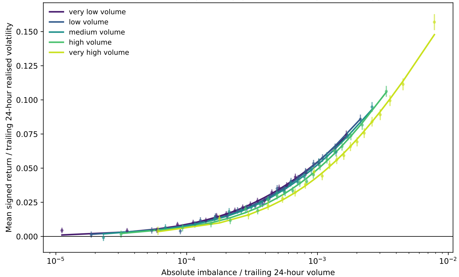
4,000-event bars: response by gross-volume regime (full support)
