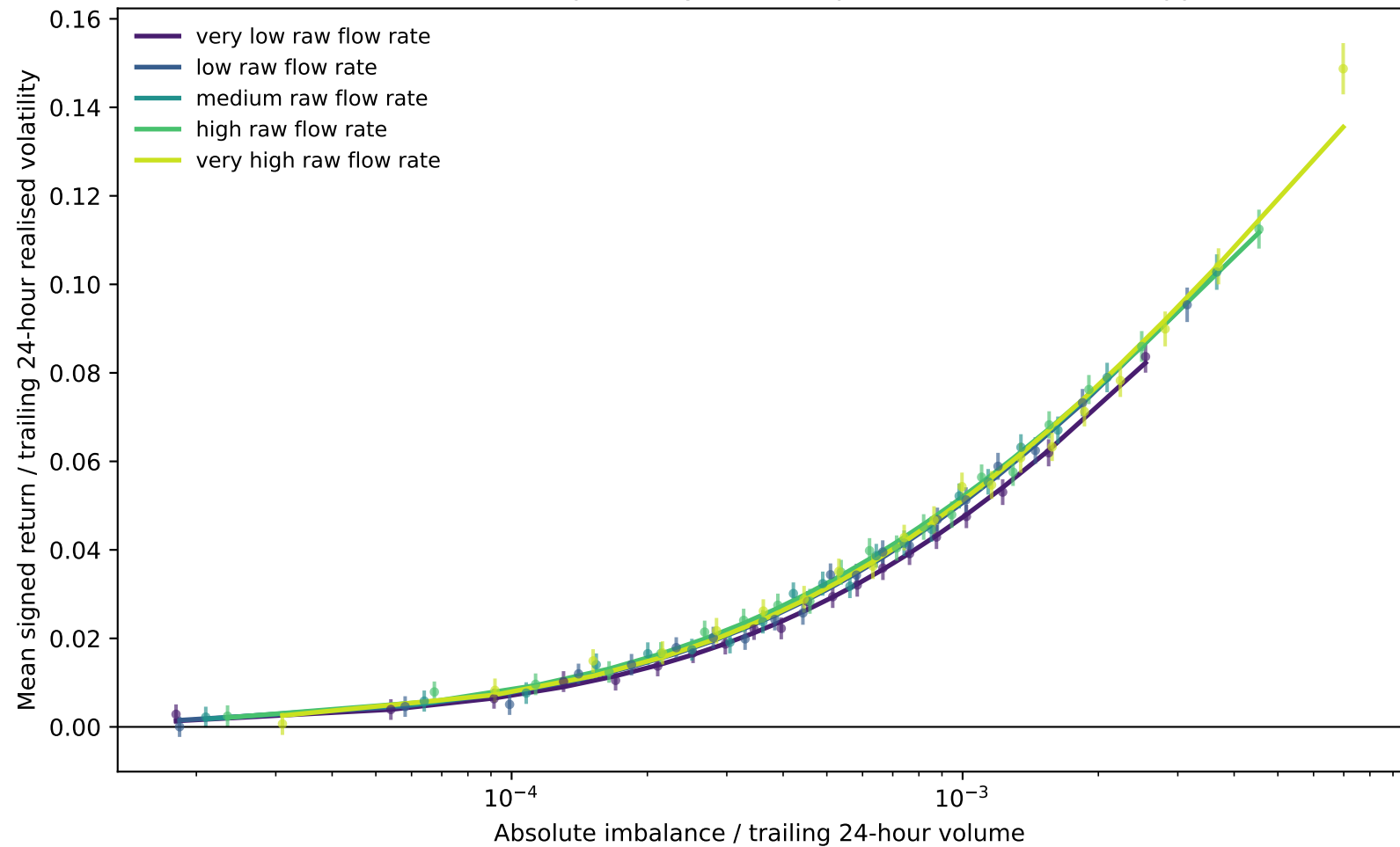
4,000-event bars: response by raw BTC-per-second flow (full support)
