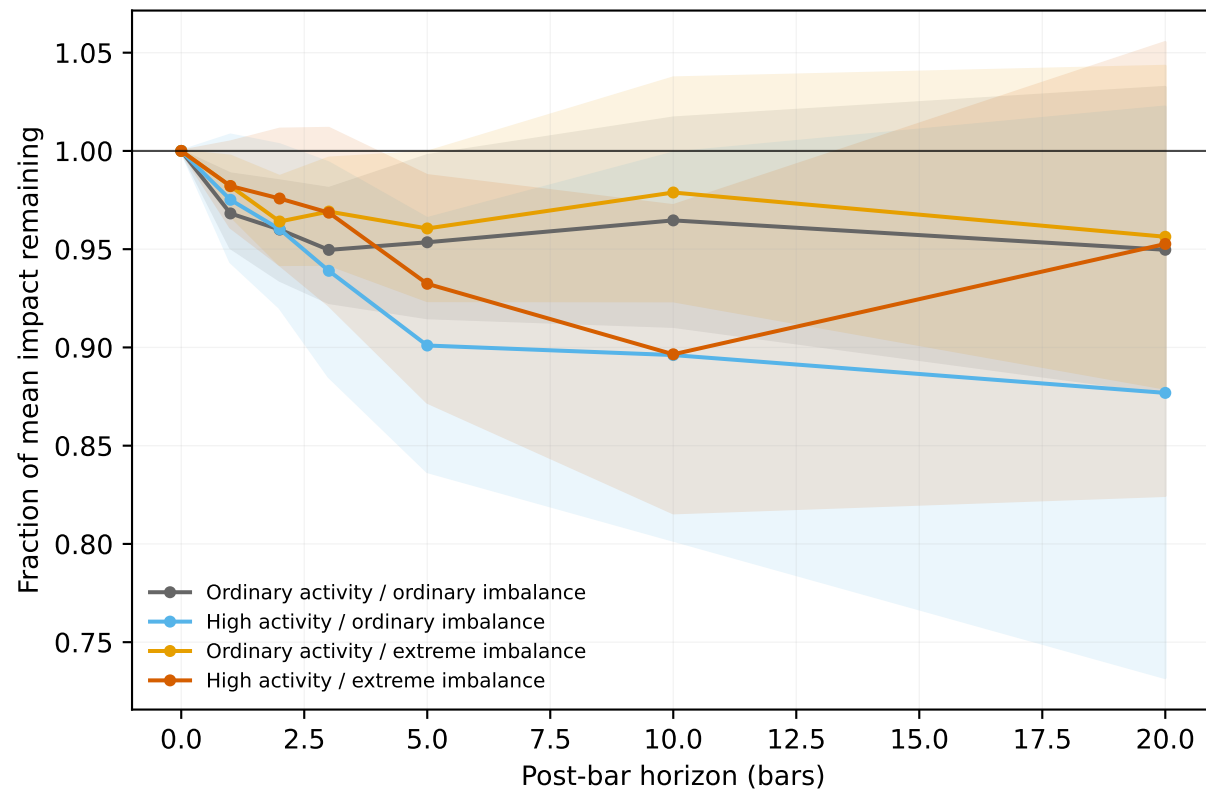
4,000-event bars
