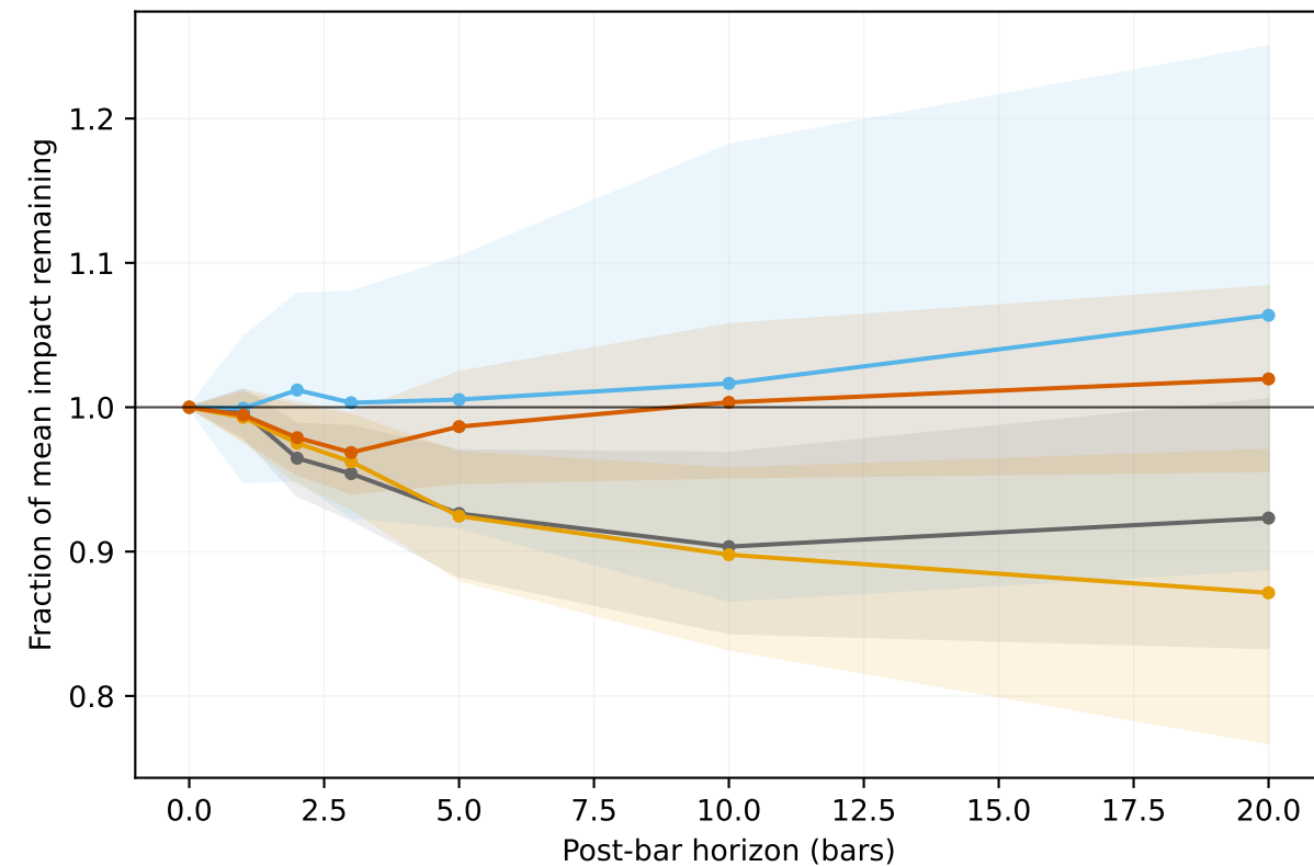
Five-minute bars
