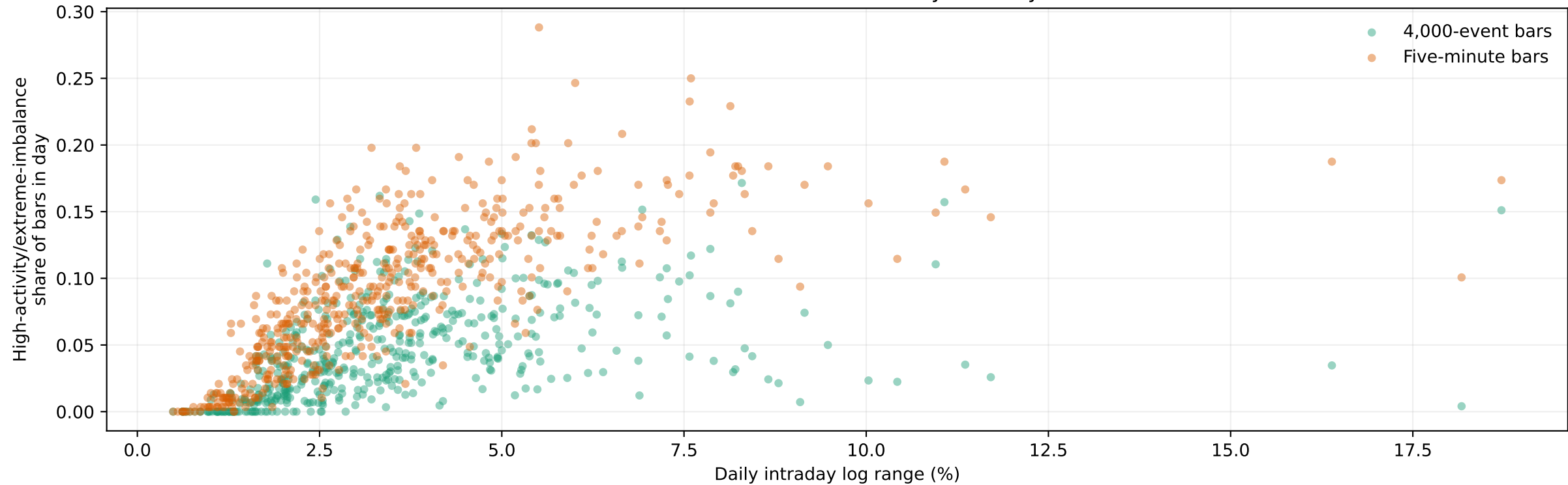
State concentration and daily volatility
