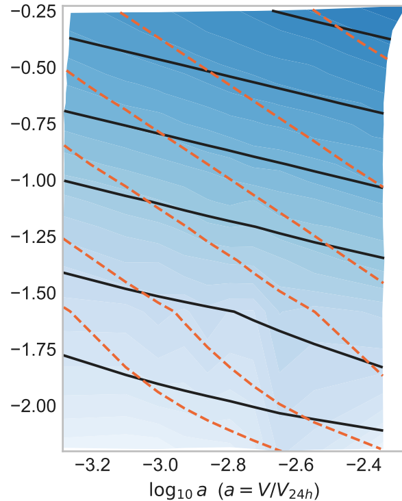
N = 2,000 events
