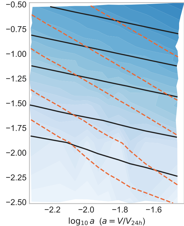
N = 16,000 events
