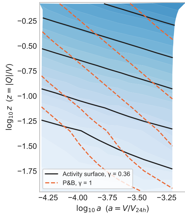
N = 250 events
