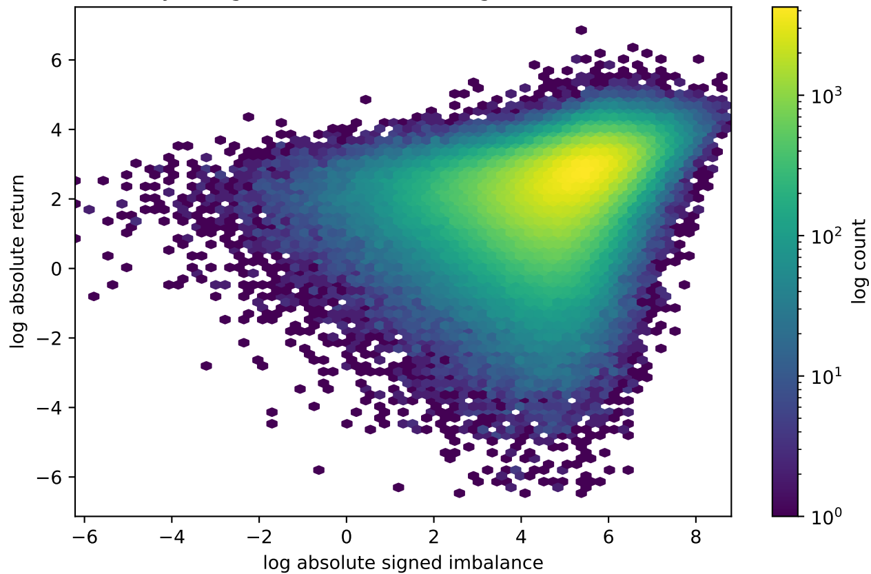
Density of log absolute return vs log absolute imbalance
