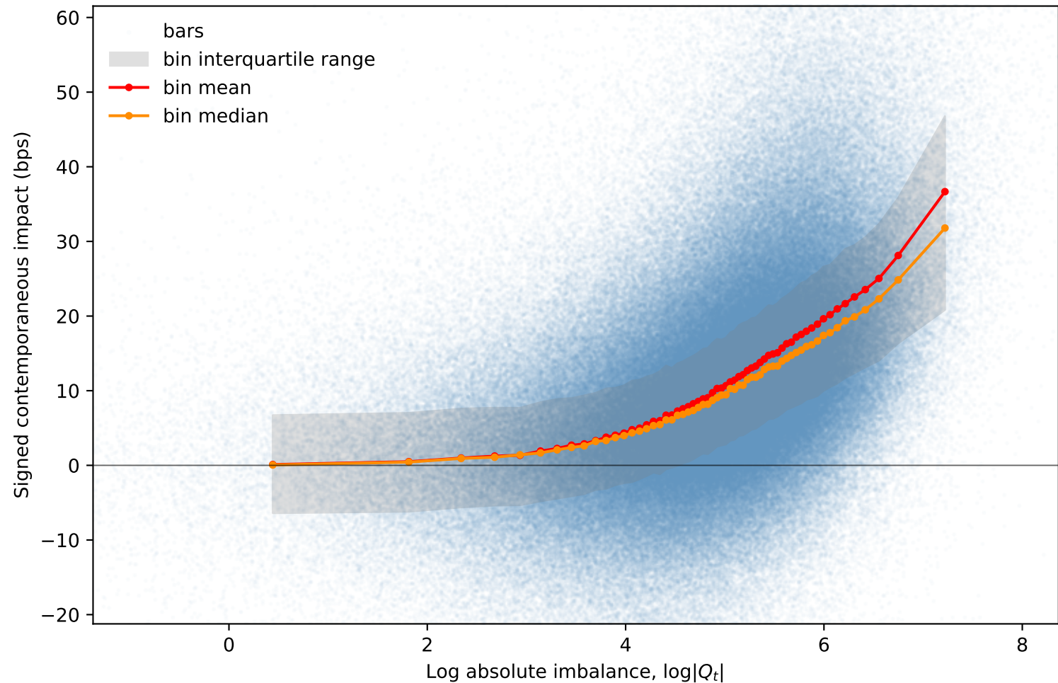
Signed impact conditional on absolute imbalance
