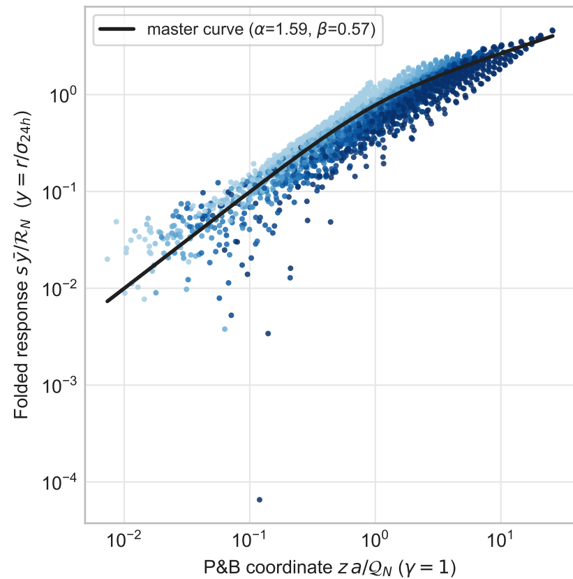
P&B ( \gamma = 1 ): weighted RMSE 20.6
