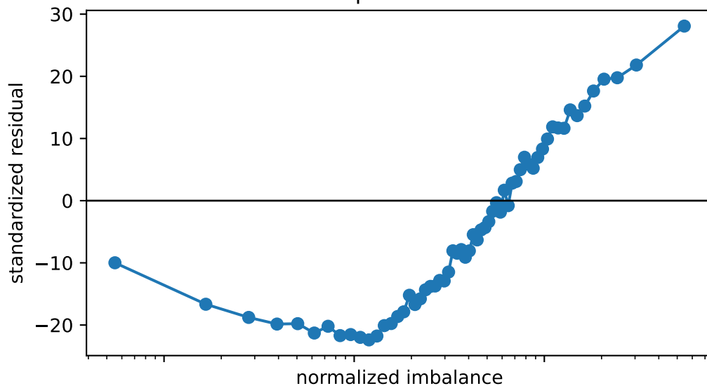
logarithmic
