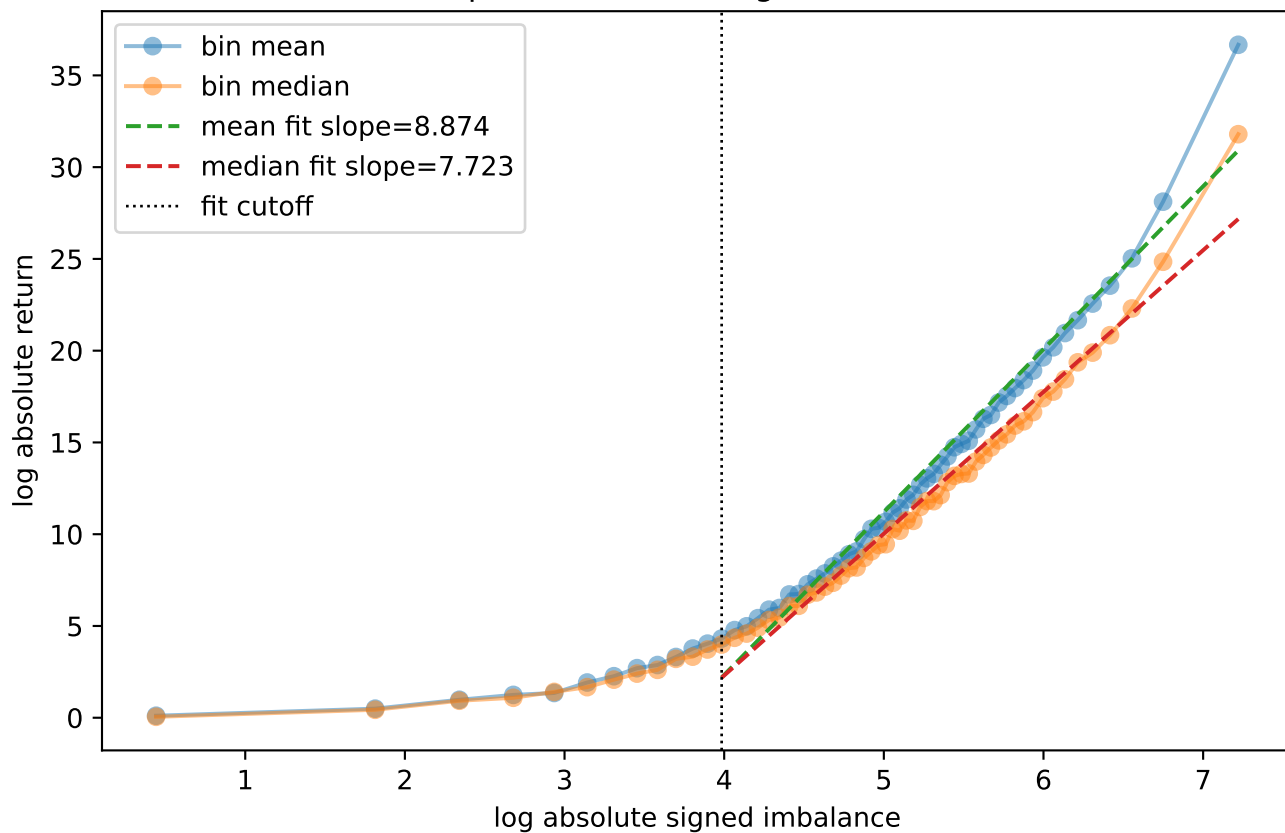
Binned slopes after excluding low-imbalance bins
