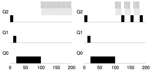
Figure 8.4: Without (Left) and With (Right) Priority Boost
