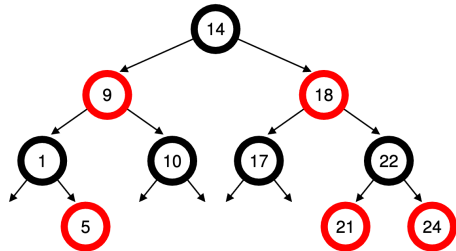
Figure 9.5: CFS Red-Black Tree
