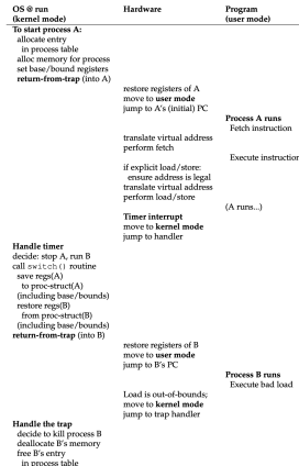
Figure 15.6: Limited Direct Execution (Dynamic Relocation) @ Runtime
