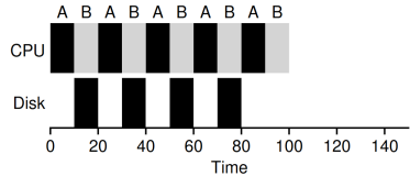
Figure 7.9: Overlap Allows Better Use Of Resources
