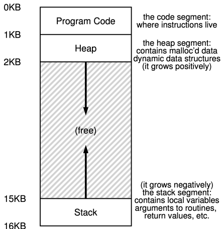
Figure 13.3: An Example Address Space
