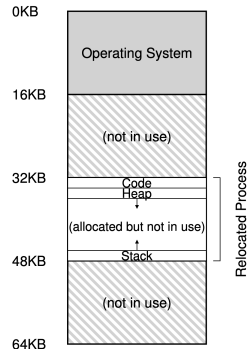
Figure 15.2: Physical Memory with a Single Relocated Process
