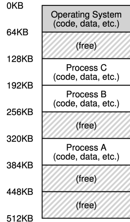
Figure 13.2: Three Processes: Sharing Memory
