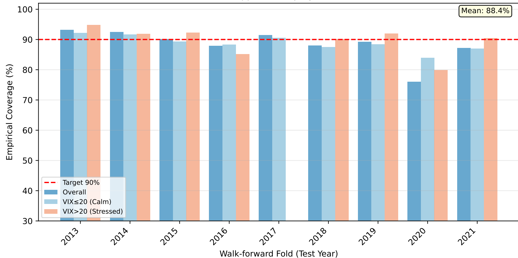
Track A — Conformal Prediction Coverage (90% Target) by VIX Regime [Supplementary figure]
