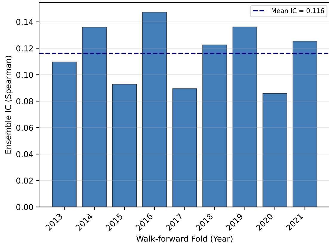
Track A — Per-Fold Ensemble IC (IS 2013-21)
