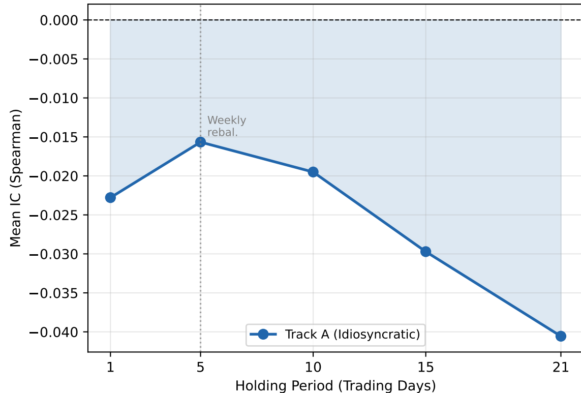
Track A — IC Decay vs Horizon
