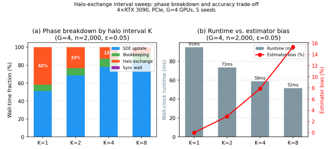
Figure 2: Halo-exchange interval sweep ( G=4 RTX 3090 PCIe, n=2,000 , \varepsilon=0.05 , 5 seeds). Left : stacked phase breakdown showing the fraction of wall time in each component (SDE update, MLMC bookkeeping, halo/all-reduce, sync wait) for K=1, 2, 4, 8 . At K=1 the halo phase accounts for 41.7% of total runtime; K=2 halves this to 23.5%, proportionally increasing SDE compute time. Right : runtime (bars) and estimator bias (red line) as functions of K , showing the accuracy–efficiency trade-off. K=2 offers 22.5% runtime reduction at only 2.9% bias.
