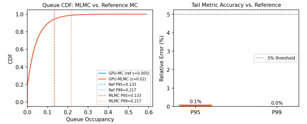
FIGURE 2: Tail-delay validation on a synthetic Erdős-Rényi network ( n = 500 , \varepsilon = 0.02 ). GPU-MLMC estimates P95 and P99 queue occupancy with < 0.2\% relative error versus a tight GPU-MC reference ( \varepsilon = 0.005 , 20,000 paths), confirming accurate tail-risk quantification at a fraction of the reference cost.
